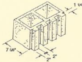
8 x 8 x 16 Scored *202*
