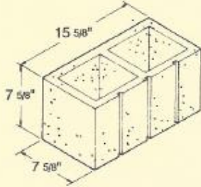
8 x 8 x 16 503 Score
