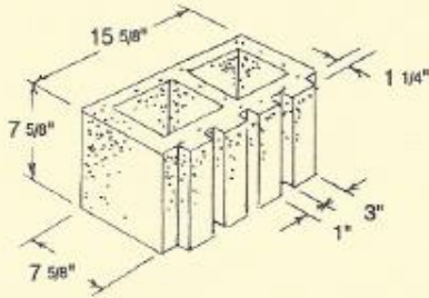
8 x 8 x 16 Scored *301*
