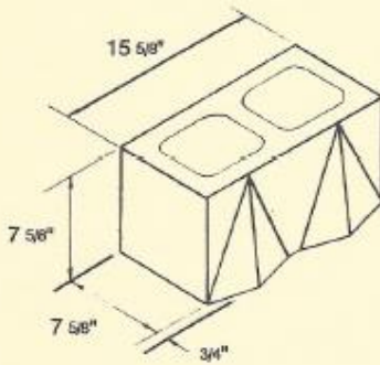
8816 MK II Also available As Single Offset Diamond
